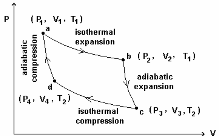
Carnot cycle
